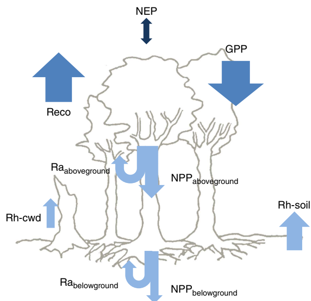
Figure 1 | Schematic representation of the major components of the forest carbon cycle. R_{a,aboveground} and R_{a,belowground} : above- and below-ground autotrophic respiration, respectively (their sum is indicated as R_a ); R_{h-soil} and R_{h-cwd} : heterotrophic respiration from soil and coarse woody debris, respectively (their sum is indicated as R_h ); NPP_{aboveground} and NPP_{belowground} : above- and belowground net primary production, respectively (their sum is indicated as NPP ); Reco : ecosystem respiration ( Reco = R_a + R_h ); GPP : gross primary production ( GPP = NPP + R_a ), and NEP : net ecosystem production ( NEP = GPP - Reco = NPP - R_h ). Each flux is associated with an arrow. Arrows pointing down indicate carbon (C) uptake, arrows pointing up indicate C release, whereas the up-down arrow indicates that both C release and C uptake can occur. The dark blue arrow indicates NEP, the mid-blue arrows indicate the primary components of NEP ( Reco and GPP ), whereas the light blue arrows indicate the components of Reco and GPP .
