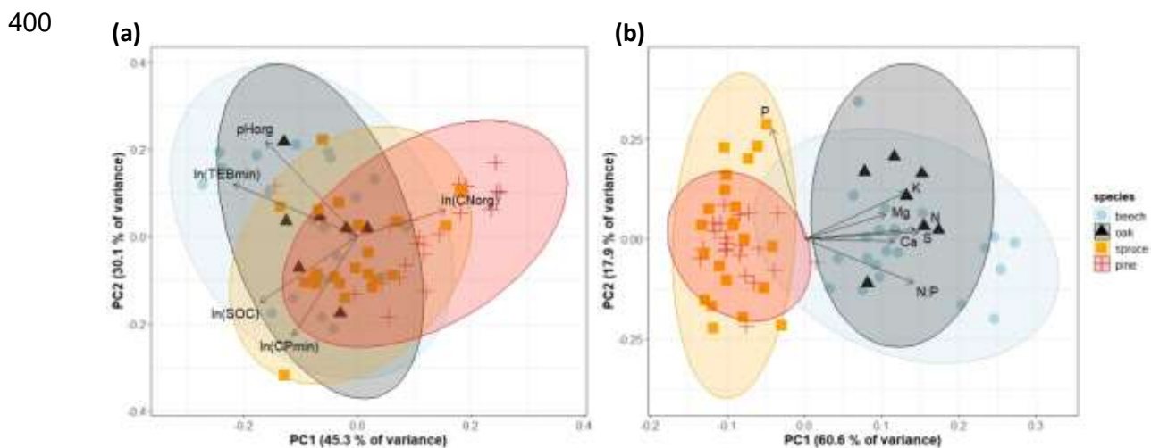
Figure 3 Principal component analysis on (a) key soil variables (sd for PC1 = 1.51, sd for PC2 = 1.23), and (b) foliar stoichiometry data in the European ICP Forests dataset (sd for PC1 = 2.06, sd for PC2 = 1.12). These soil variables in particular were chosen because of their link with the soil nutrient status (e.g. Van Sundert et al., 2018), and our observation during exploratory analyses that organic layer characteristics in particular explain
