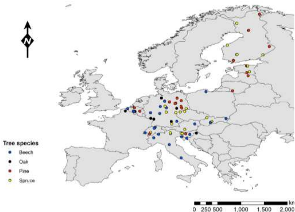
Figure 2 Location of the 77 ICP Forests sites used for the main analyses in this study. Dominant tree species growing on the sites were Common beech ( Fagus sylvatica L.), Pedunculate oak ( Quercus robur L.), Scots pine ( Pinus sylvestris L.) or Norway spruce ( Picea abies (L.) H. Karst.).
