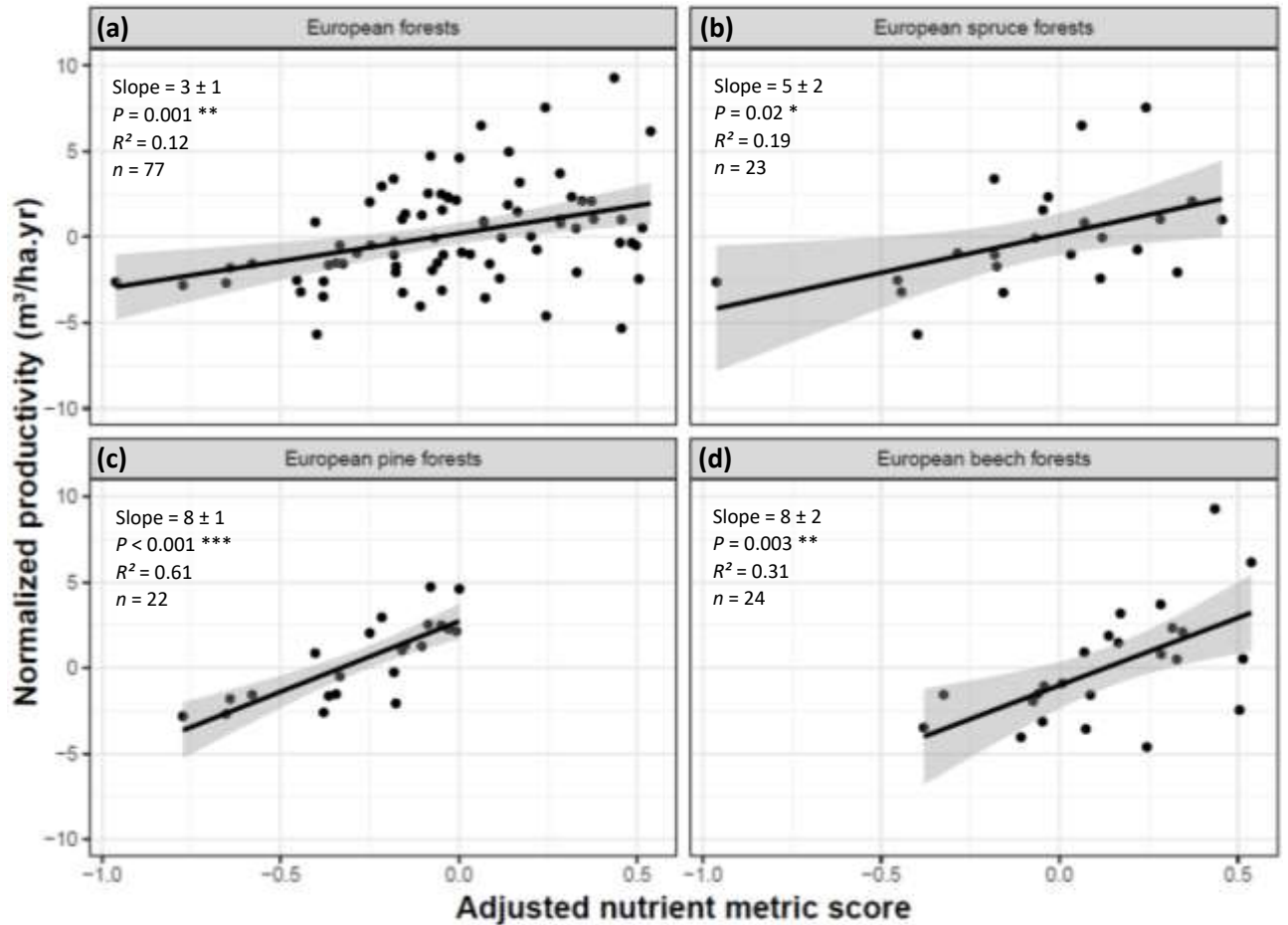
605 Figure 4 Normalized productivity versus the adjusted soil nutrient metric for (a) all forests, (b) spruce forests, 610 (c) pine forests and (d) beech forests. Errors on the slope estimates represent the s.e.m. Shaded areas around 615 the regression lines represent 95% confidence intervals. 620 625
