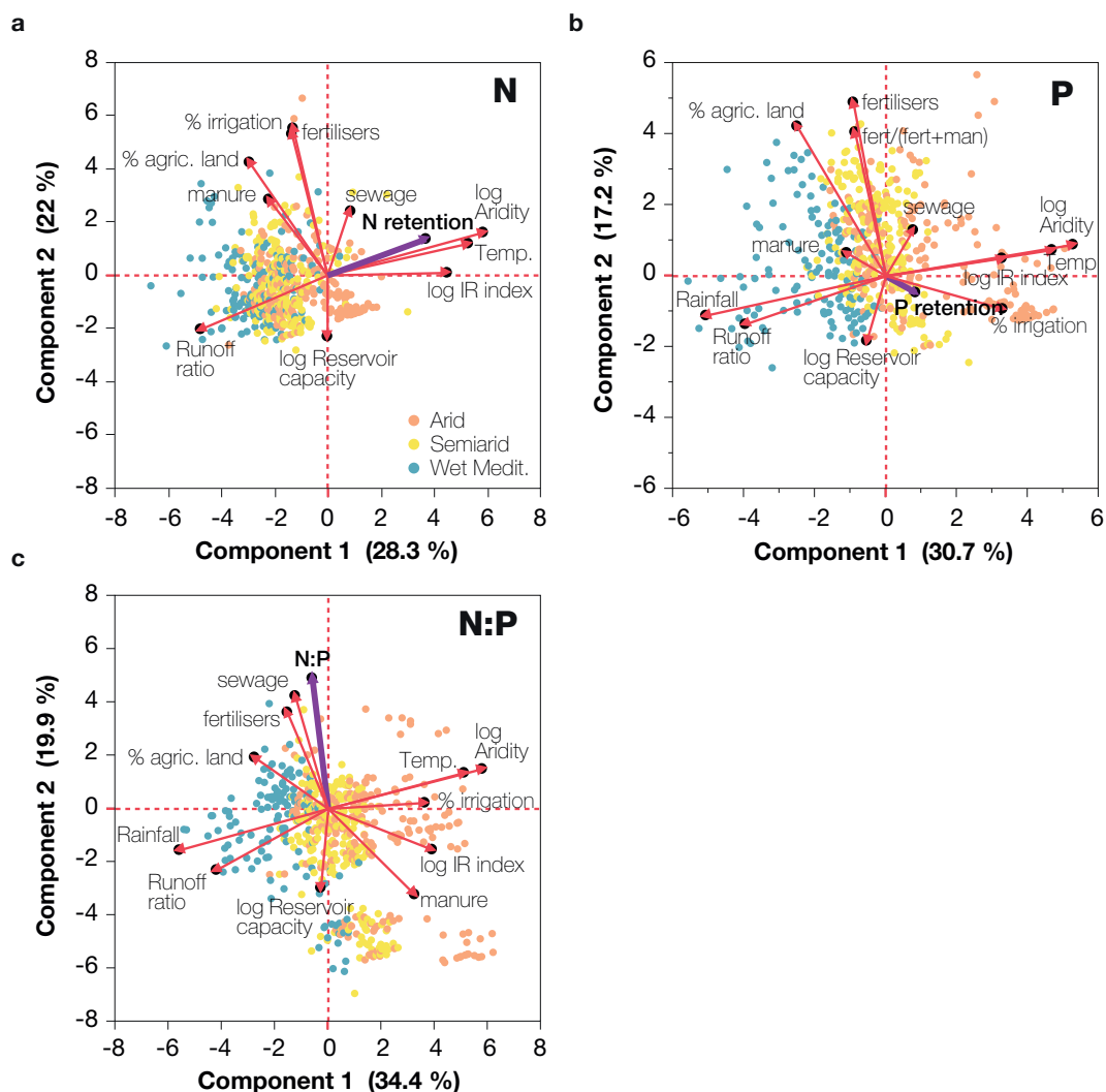
Figure 4. Main factors related to N and P retention. Principal Component Analysis for (a) N data, (b) P data, and (c) the two N, P data sets, and the N:P ratio of the inland retained nutrients. Climatic factors (temperature, rainfall, runoff ratio, aridity), water management factors (reservoir capacity, IR index, % irrigation), and terrestrial factors (synthetic fertilizers, manure, % of agricultural land, sewage) were considered in the analyses. River basins are colored according to their hydro-climatic features.
